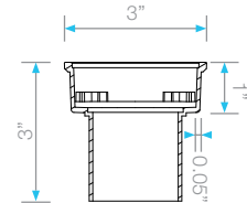
D Base - Side View
